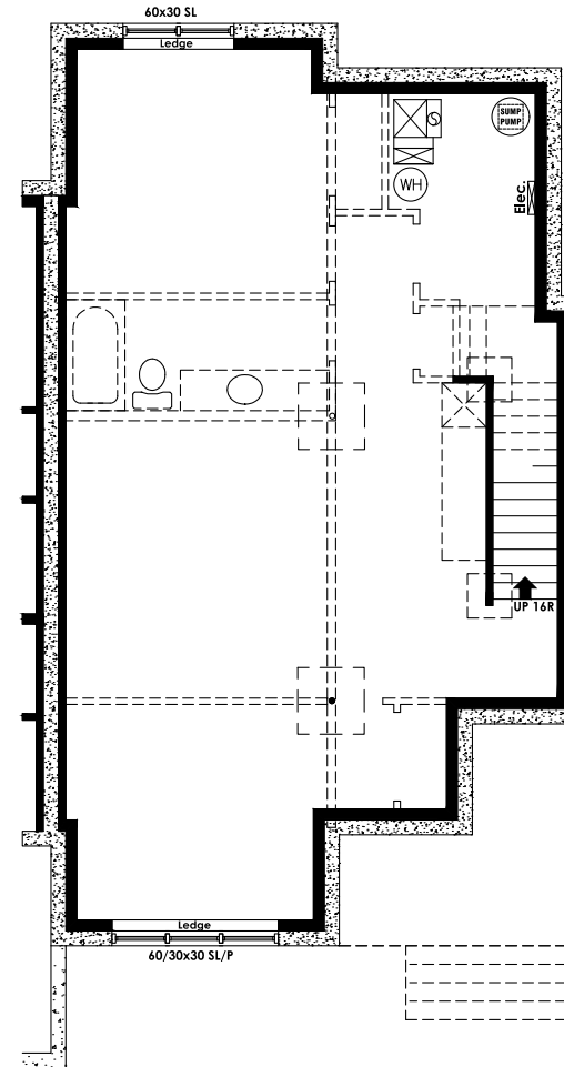
Basement Plan
