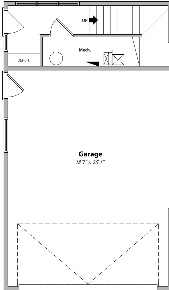
Garage Level 653 sq.ft.
