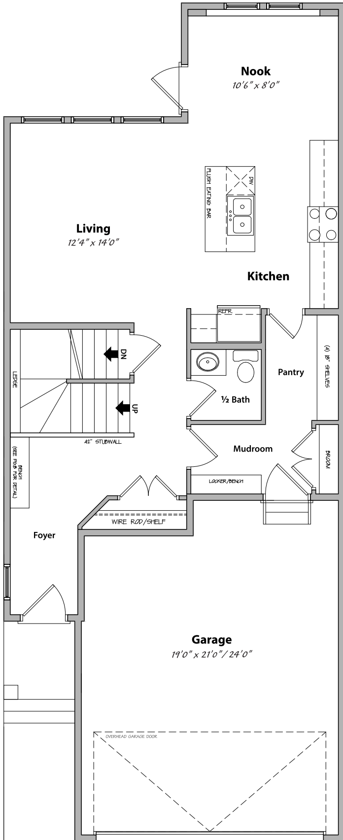
Main Level 808 sq.ft.
